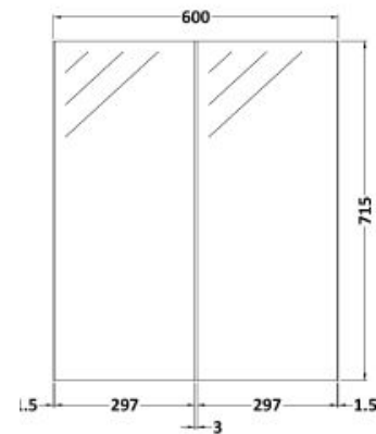
Mirror unit
