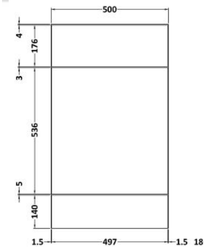
WC unit
