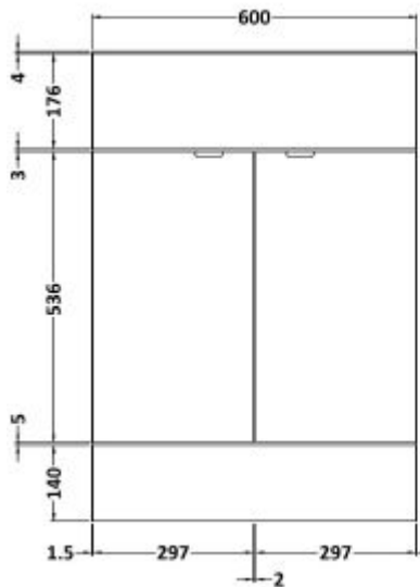
Vanity unit
