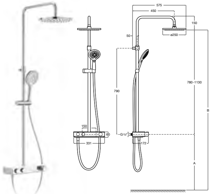
A5A9I09C00 Shower column
