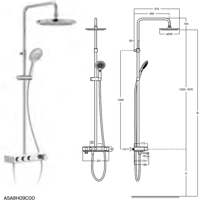
A5A9H09C00 Bath-Shower column
