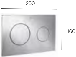
PL10 flush plate Dual flush
